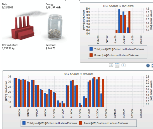
Croton on Hudson Firehouse Solar System Operation
